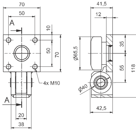
Rolle / Roller XSTR 060.6200
