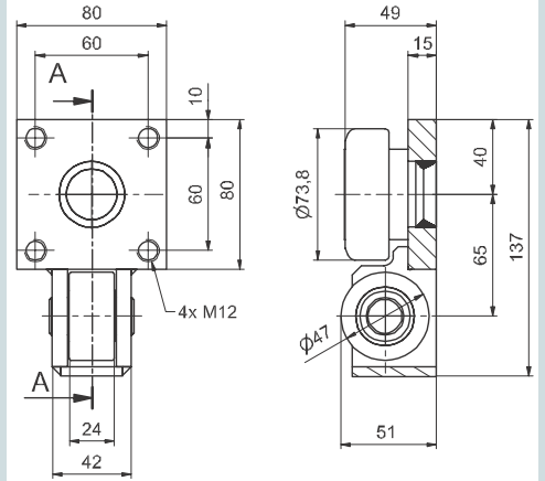
Rolle / Roller XSTR 070.6200
