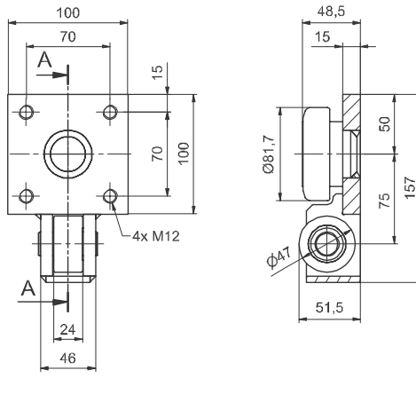
Rolle / Roller XSTR 080.6200
